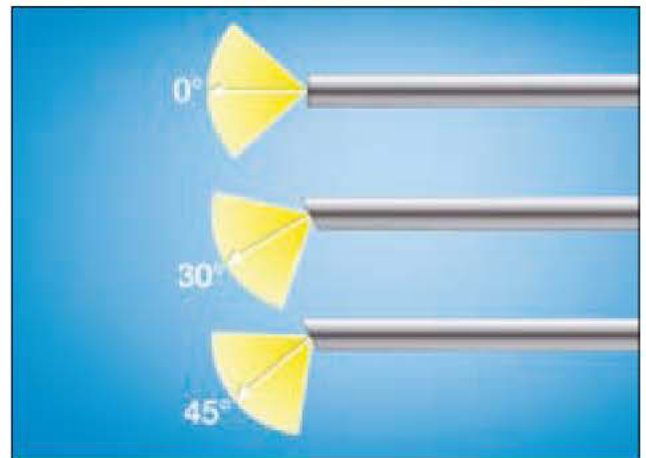
Fig. 28 HOPKINS® rod-lens laparoscopes are available with different angles of view.
