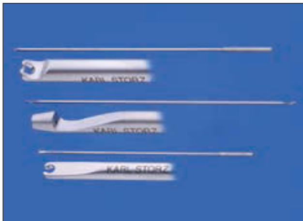
Fig. 53 Knot tier for extracorporeal knotting. The close-up views show the various types of open-end, and closed-end tip design.
