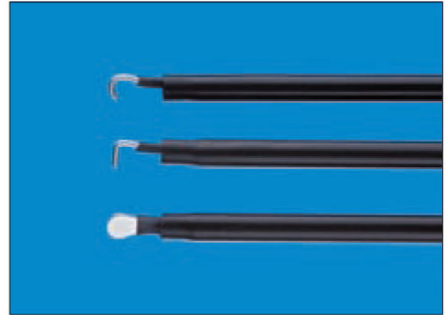
Fig. 44b Spatula- and hook-shaped unipolar electrodes.
